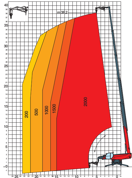
JW 2000 Jib winch 2.000 kg
