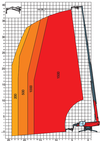
JW 1500 Jib winch 1.500 kg
