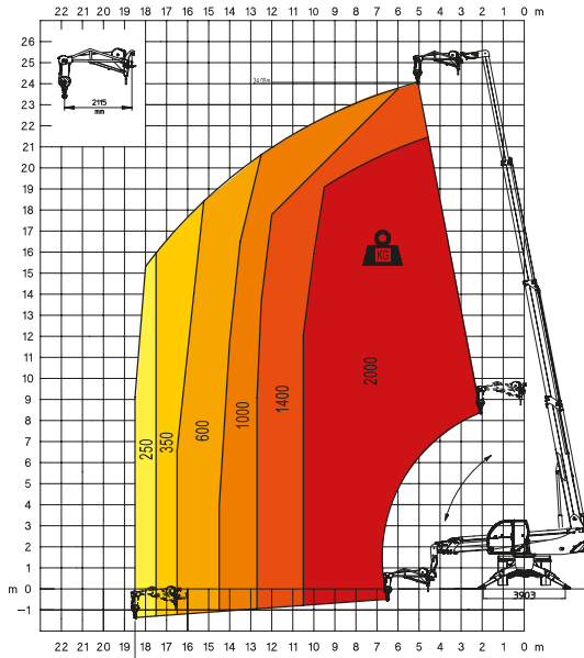
JW 2000 Jib winch 2.000
