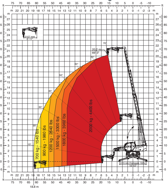
Jib winch 2.000 kg
