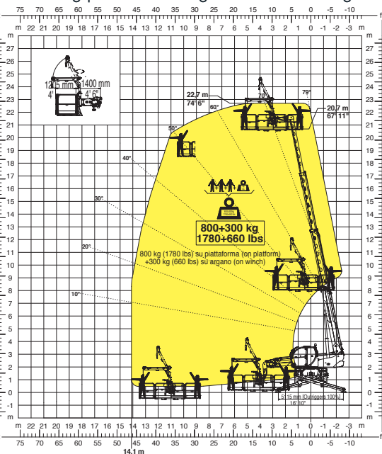
Rotating platform 800 kg with winch 300 kg
