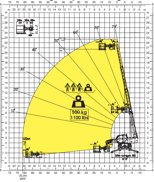
Rotating fixed platform 500 kg
