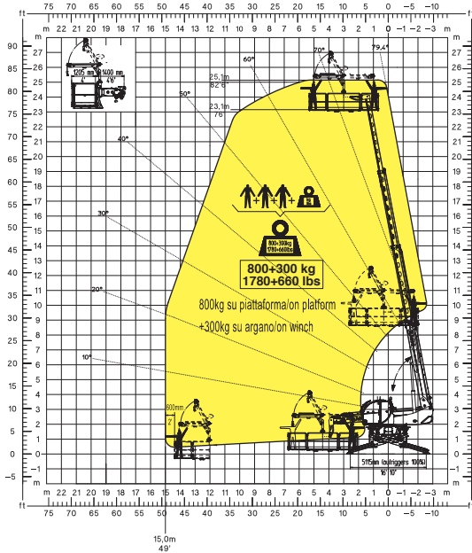
Rotating platform 800 kg with winch 300 kg
