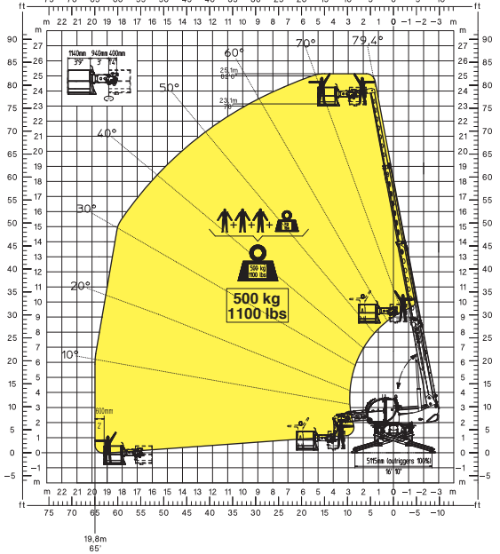
Rotating fixed platform 500 kg
